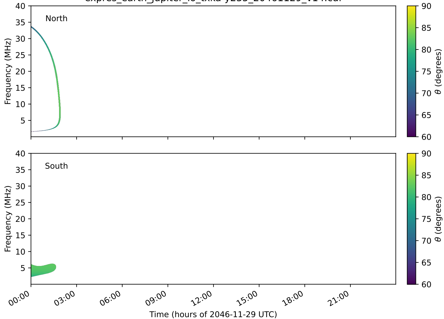
expres_earth_jupiter_io_txka-y235_20461129_v14.cdf
