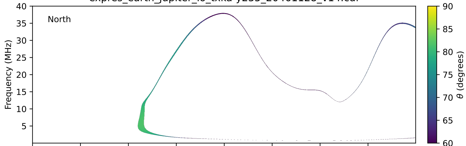
expres_earth_jupiter_io_txka-y235_20461128_v14.cdf
