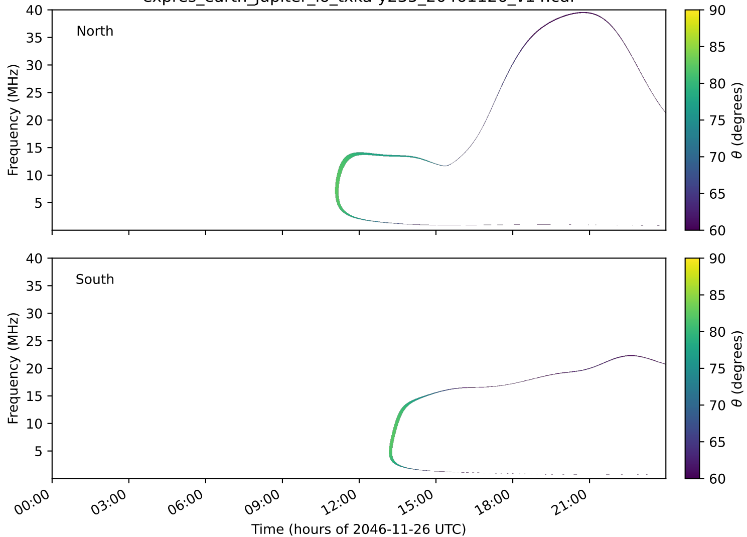
expres_earth_jupiter_io_txka-y235_20461126_v14.cdf
