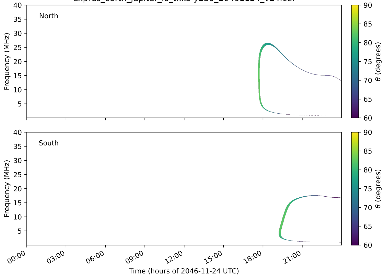
expres_earth_jupiter_io_txka-y235_20461124_v14.cdf
