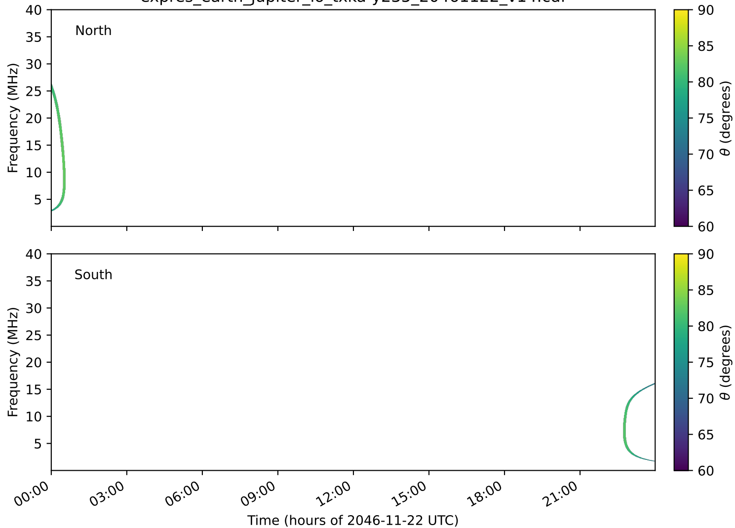
expres_earth_jupiter_io_txka-y235_20461122_v14.cdf
