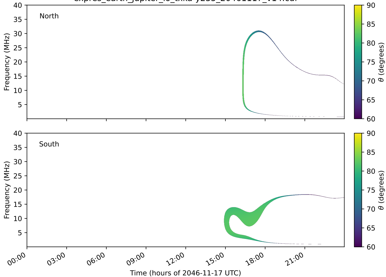
expres_earth_jupiter_io_txka-y235_20461117_v14.cdf
