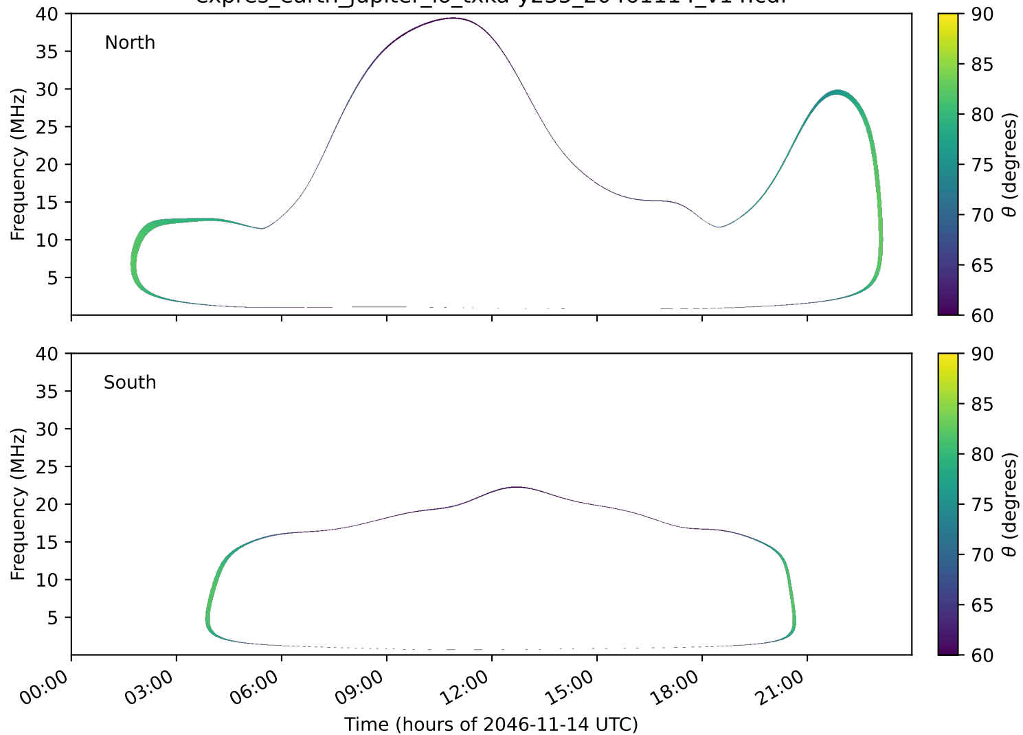
expres_earth_jupiter_io_txka-y235_20461114_v14.cdf
