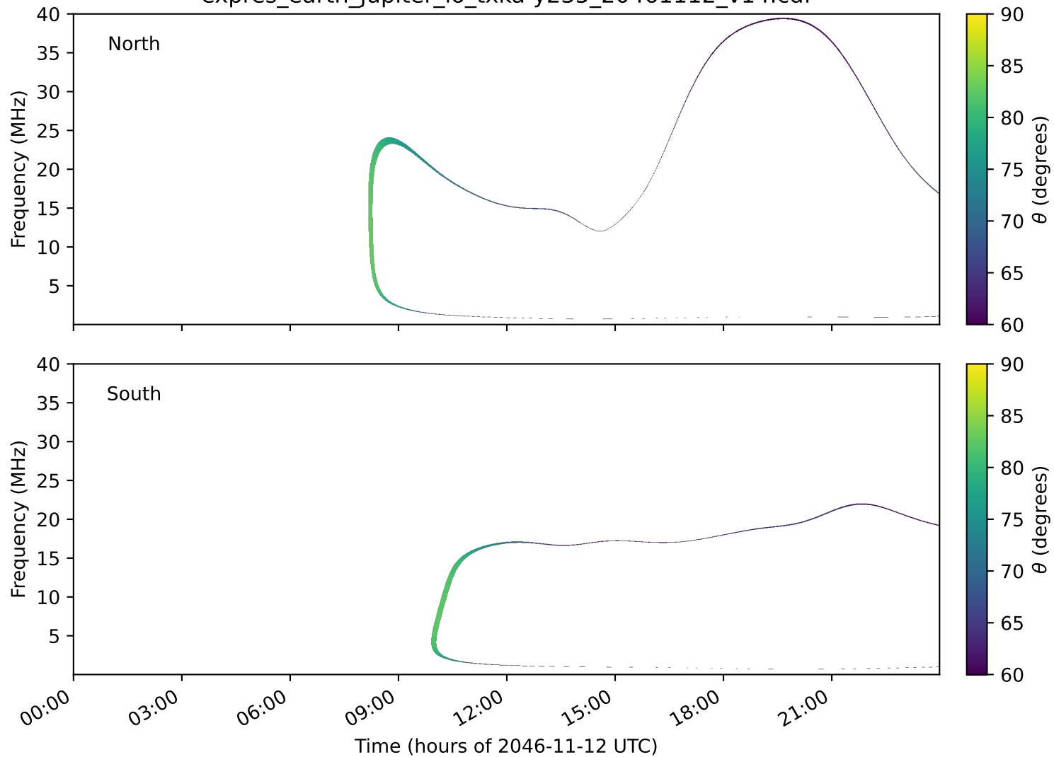
expres_earth_jupiter_io_txka-y235_20461112_v14.cdf
