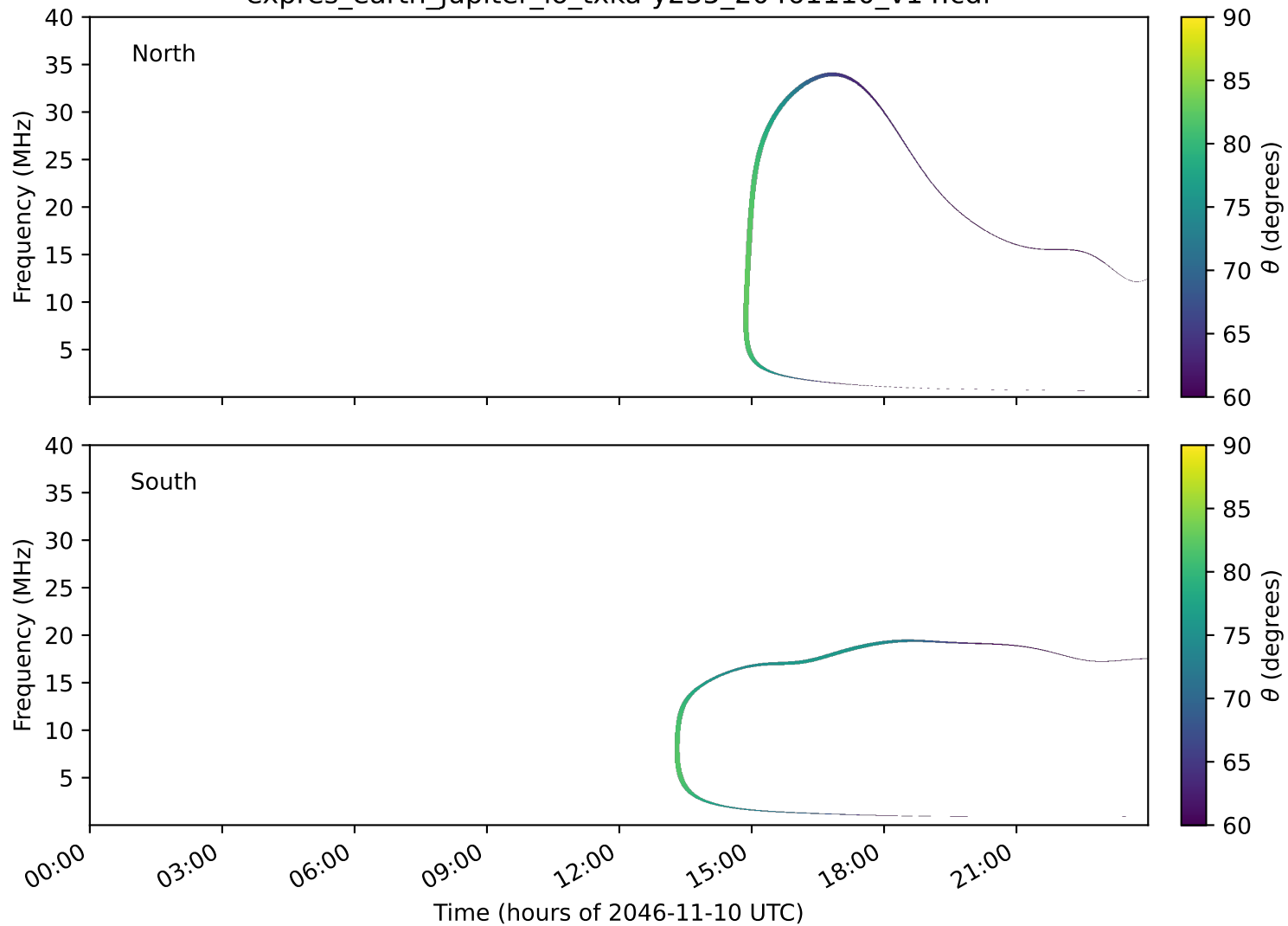
expres_earth_jupiter_io_txka-y235_20461110_v14.cdf
