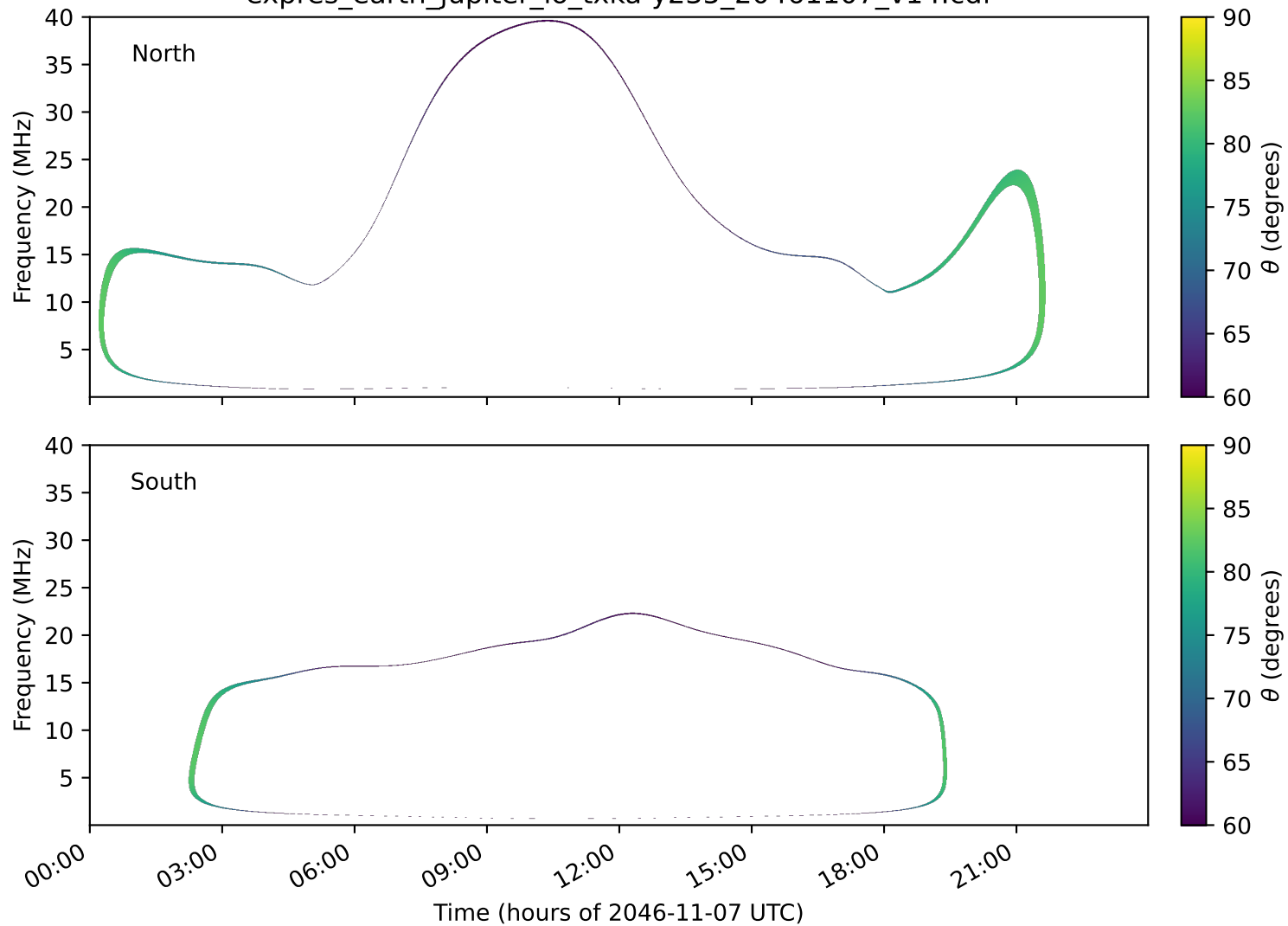
expres_earth_jupiter_io_txka-y235_20461107_v14.cdf
