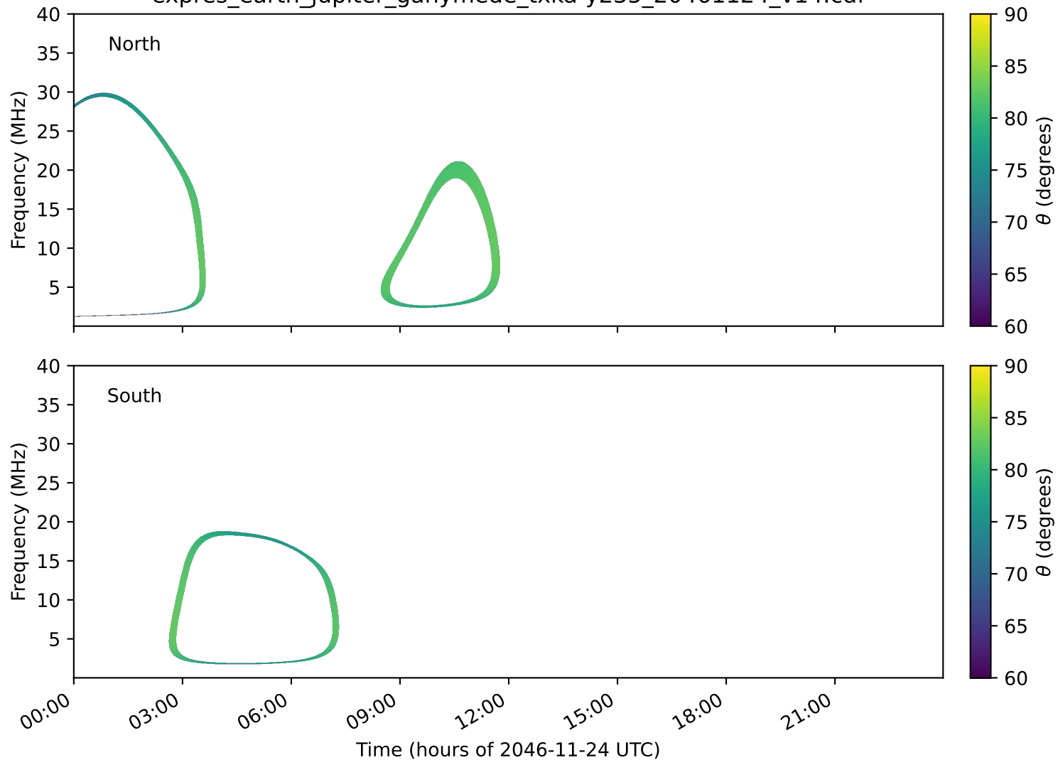
expres_earth_jupiter_ganymede_txka-y235_20461124_v14.cdf
