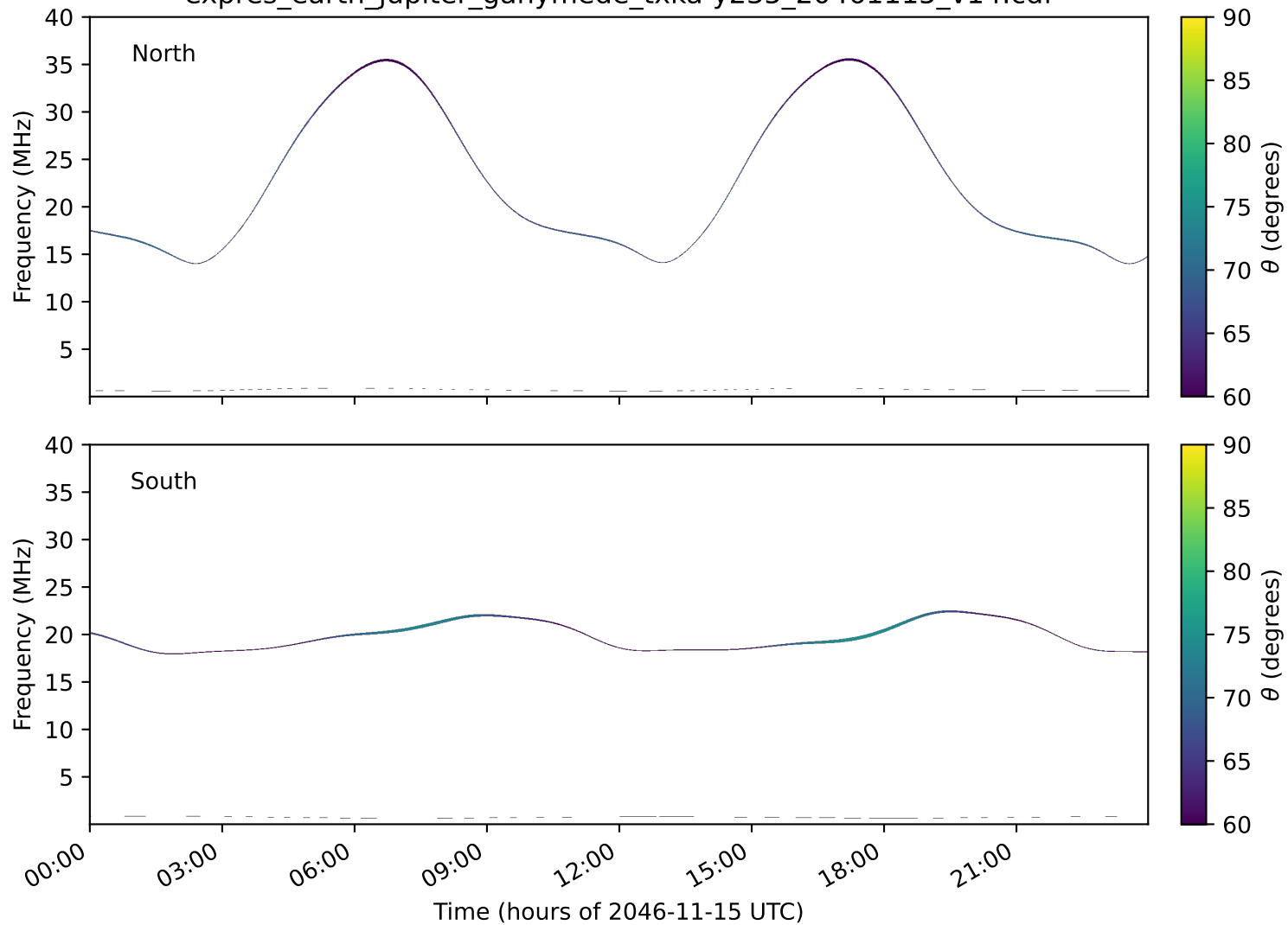
expres_earth_jupiter_ganymede_txka-y235_20461115_v14.cdf
