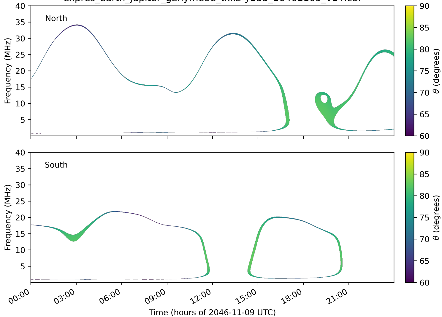
expres_earth_jupiter_ganymede_txka-y235_20461109_v14.cdf
