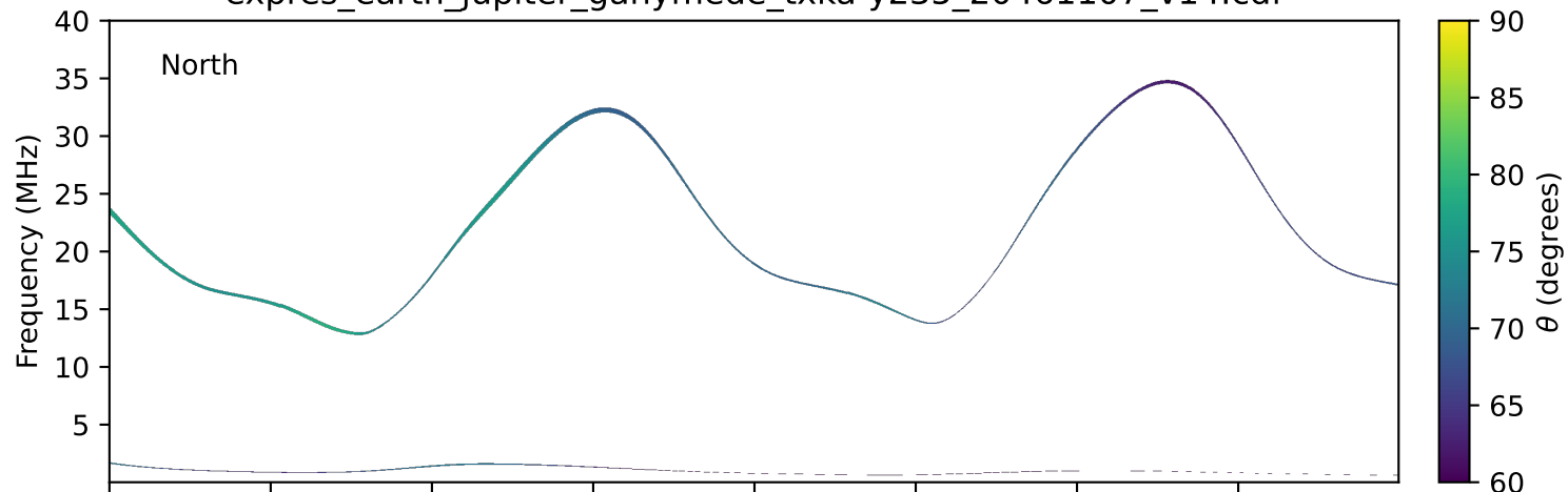
expres_earth_jupiter_ganymede_txka-y235_20461107_v14.cdf
