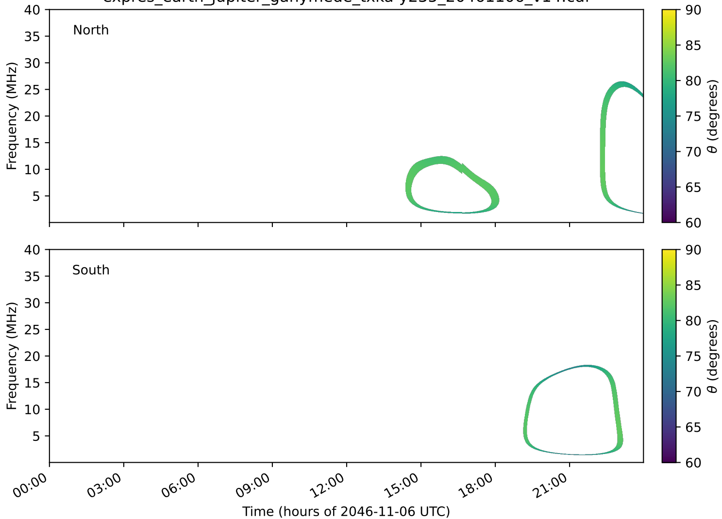
expres_earth_jupiter_ganymede_txka-y235_20461106_v14.cdf
