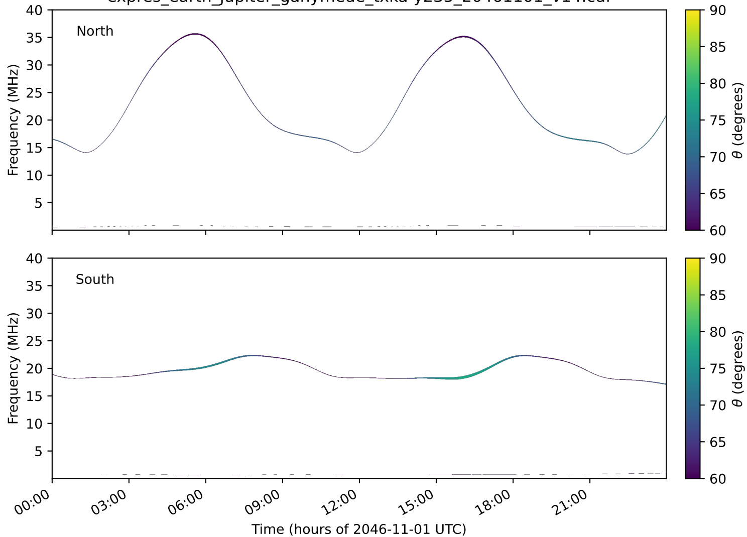
expres_earth_jupiter_ganymede_txka-y235_20461101_v14.cdf
