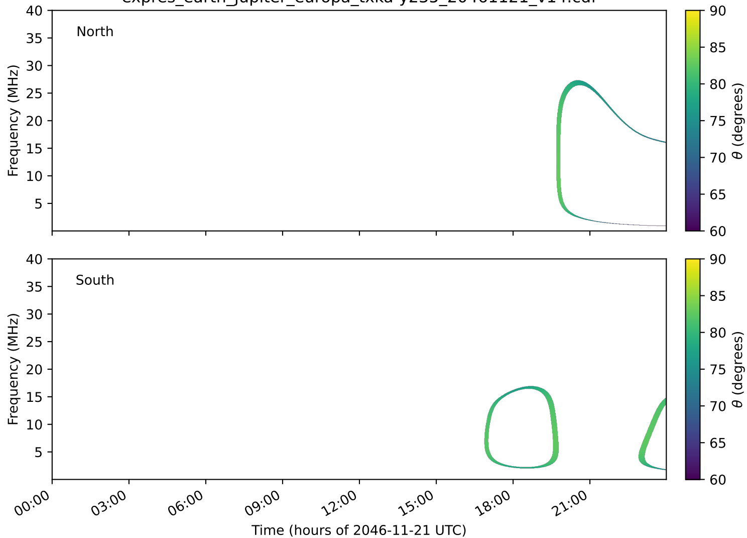
expres_earth_jupiter_europa_txka-y235_20461121_v14.cdf
