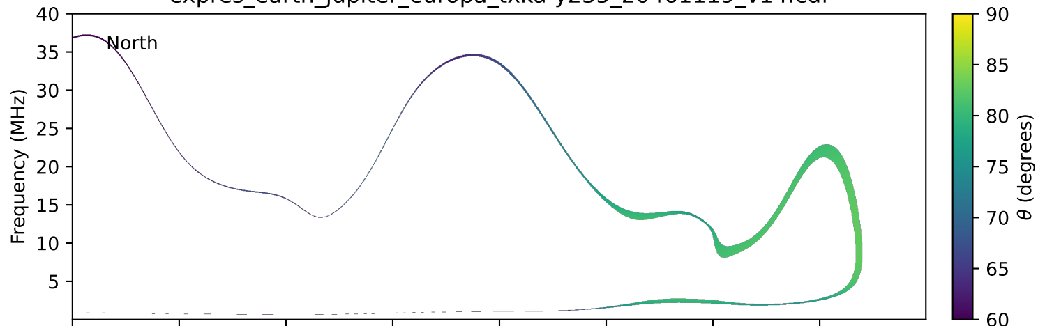
expres_earth_jupiter_europa_txka-y235_20461119_v14.cdf
