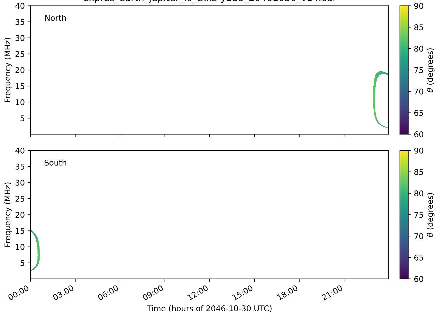
expres_earth_jupiter_io_txka-y235_20461030_v14.cdf
