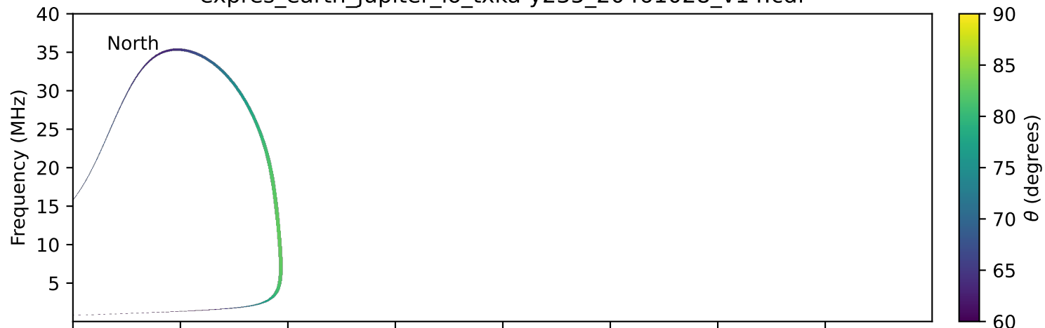
expres_earth_jupiter_io_txka-y235_20461028_v14.cdf
