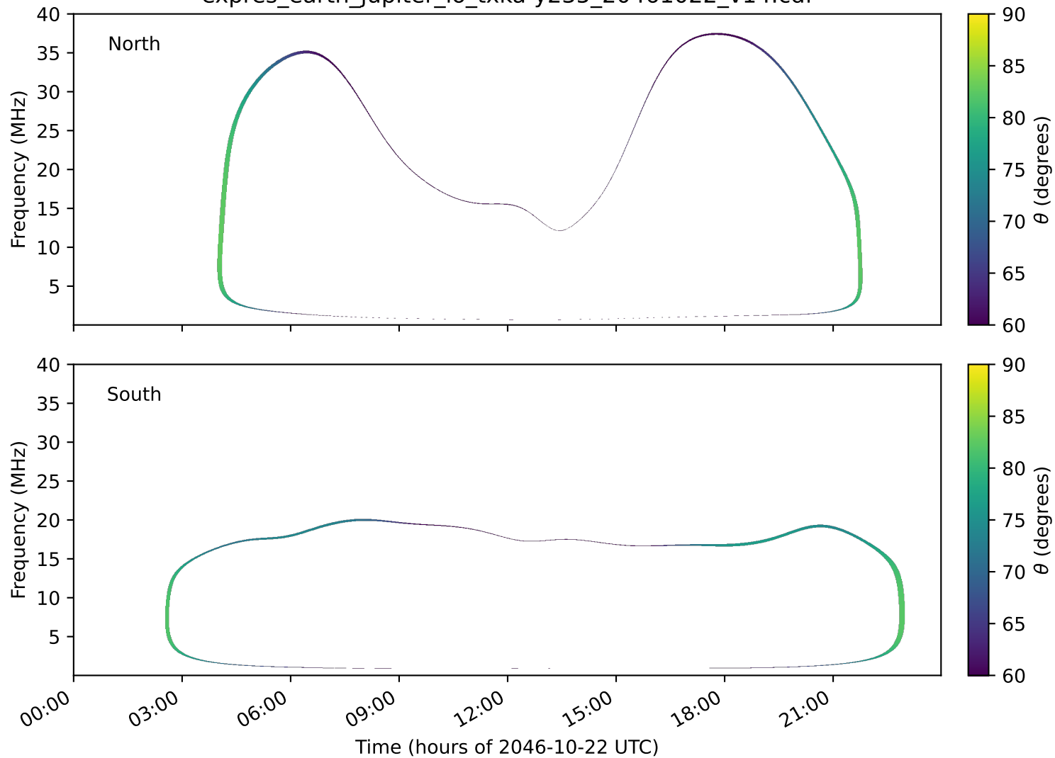
expres_earth_jupiter_io_txka-y235_20461022_v14.cdf
