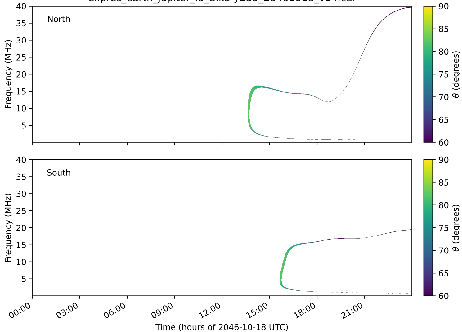
expres_earth_jupiter_io_txka-y235_20461018_v14.cdf
