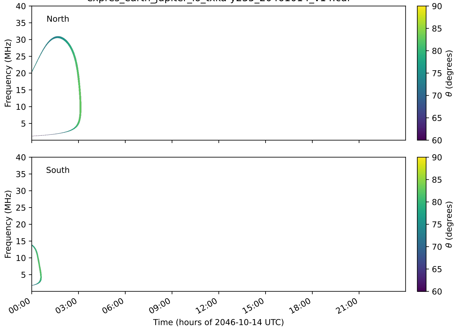
expres_earth_jupiter_io_txka-y235_20461014_v14.cdf
