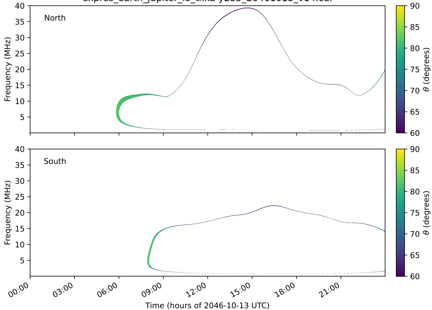
expres_earth_jupiter_io_txka-y235_20461013_v14.cdf
