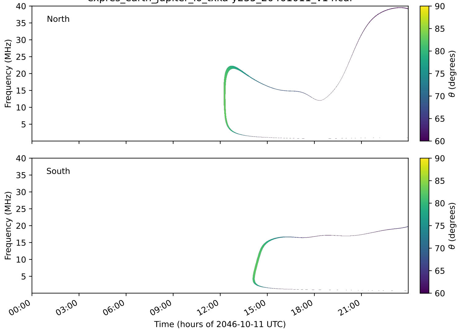
expres_earth_jupiter_io_txka-y235_20461011_v14.cdf
