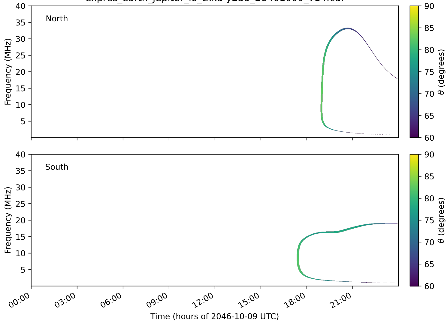
expres_earth_jupiter_io_txka-y235_20461009_v14.cdf
