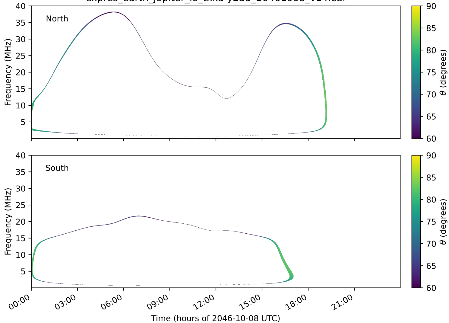
expres_earth_jupiter_io_txka-y235_20461008_v14.cdf
