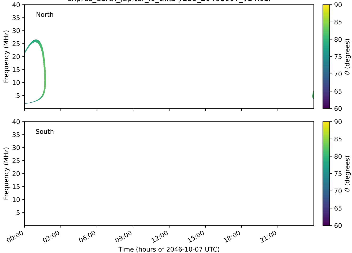
expres_earth_jupiter_io_txka-y235_20461007_v14.cdf
