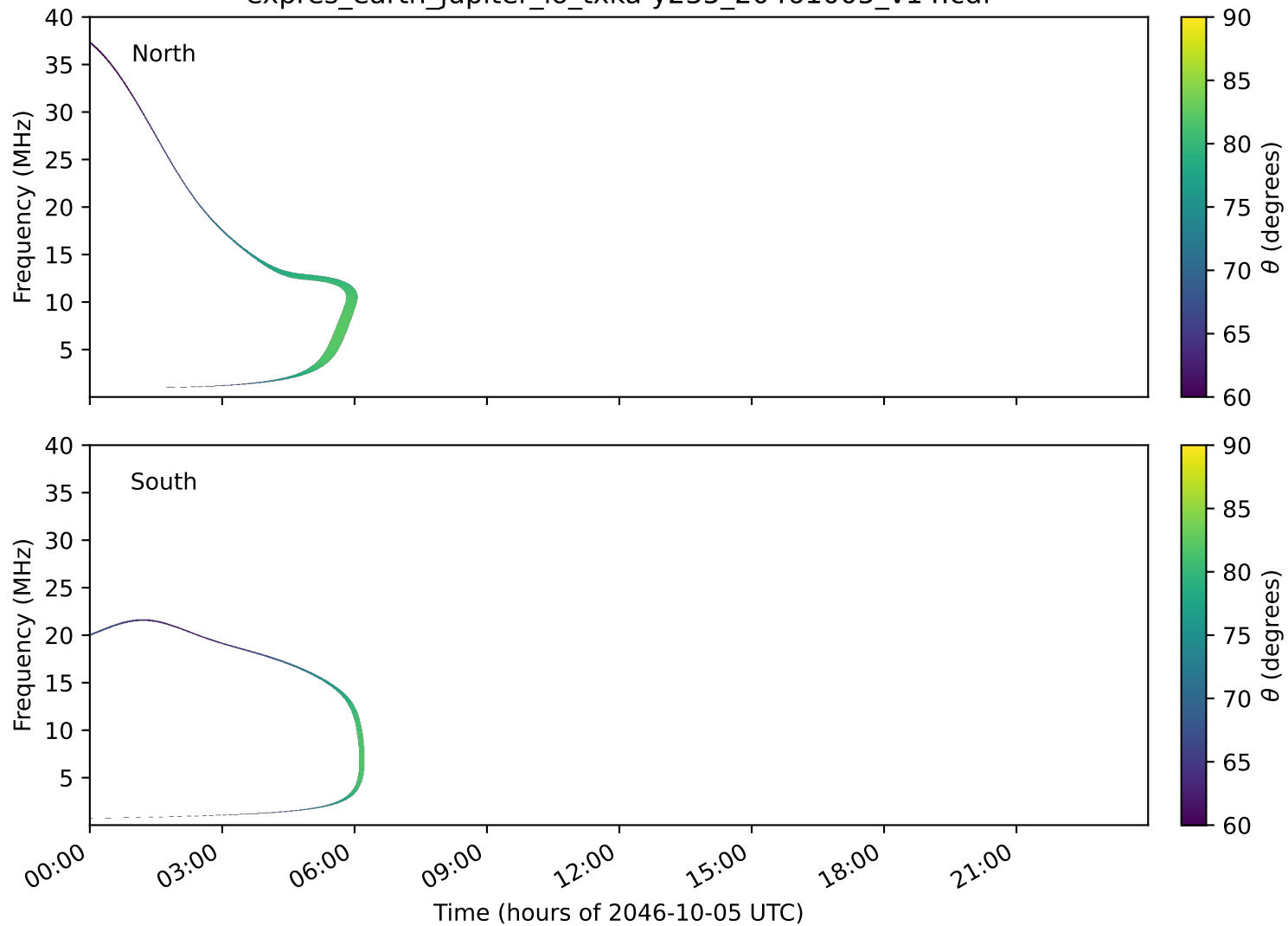
expres_earth_jupiter_io_txka-y235_20461005_v14.cdf
