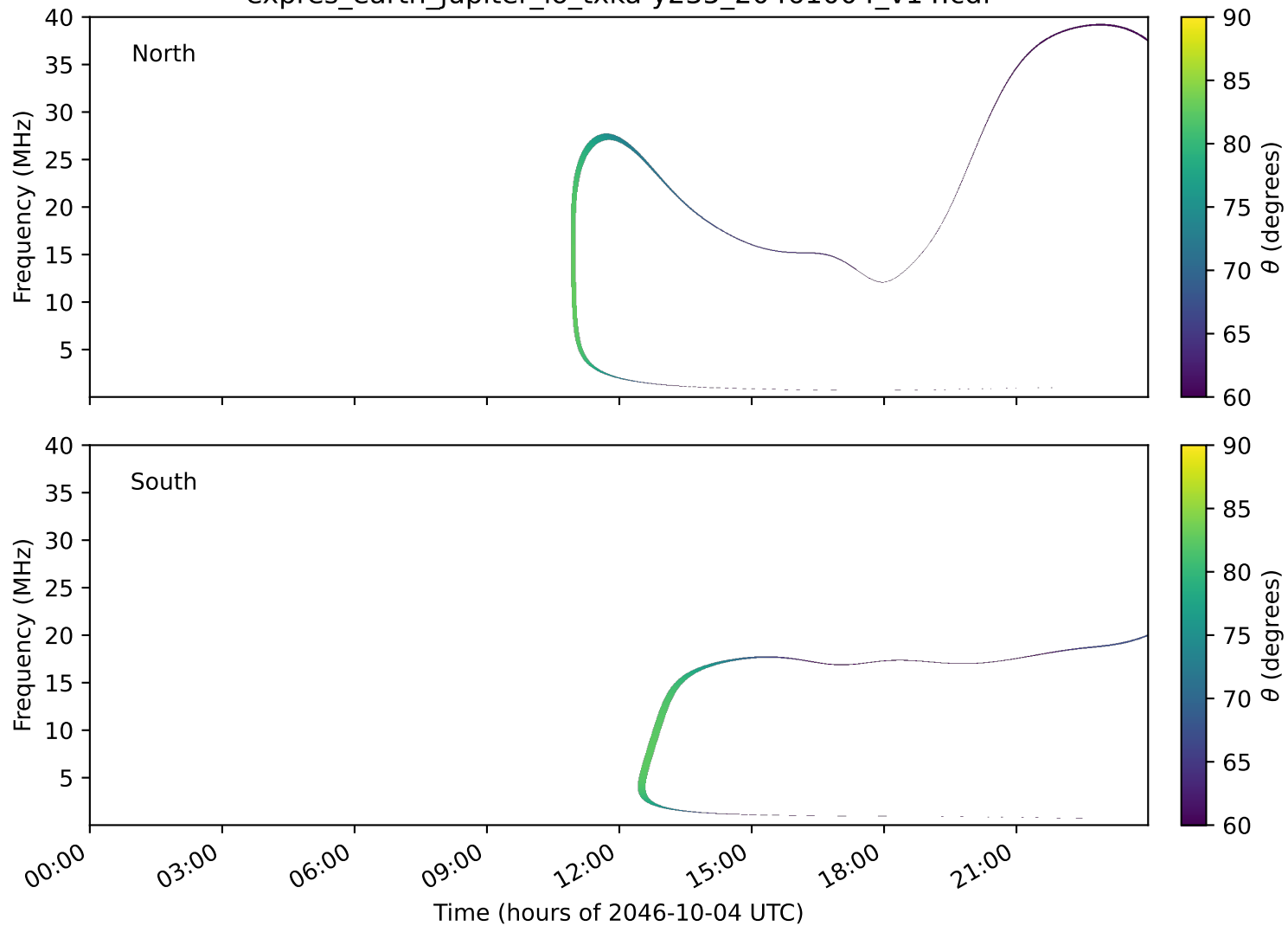
expres_earth_jupiter_io_txka-y235_20461004_v14.cdf
