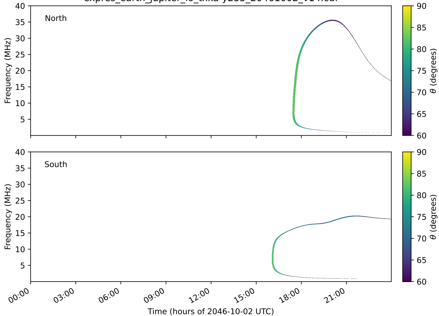
expres_earth_jupiter_io_txka-y235_20461002_v14.cdf
