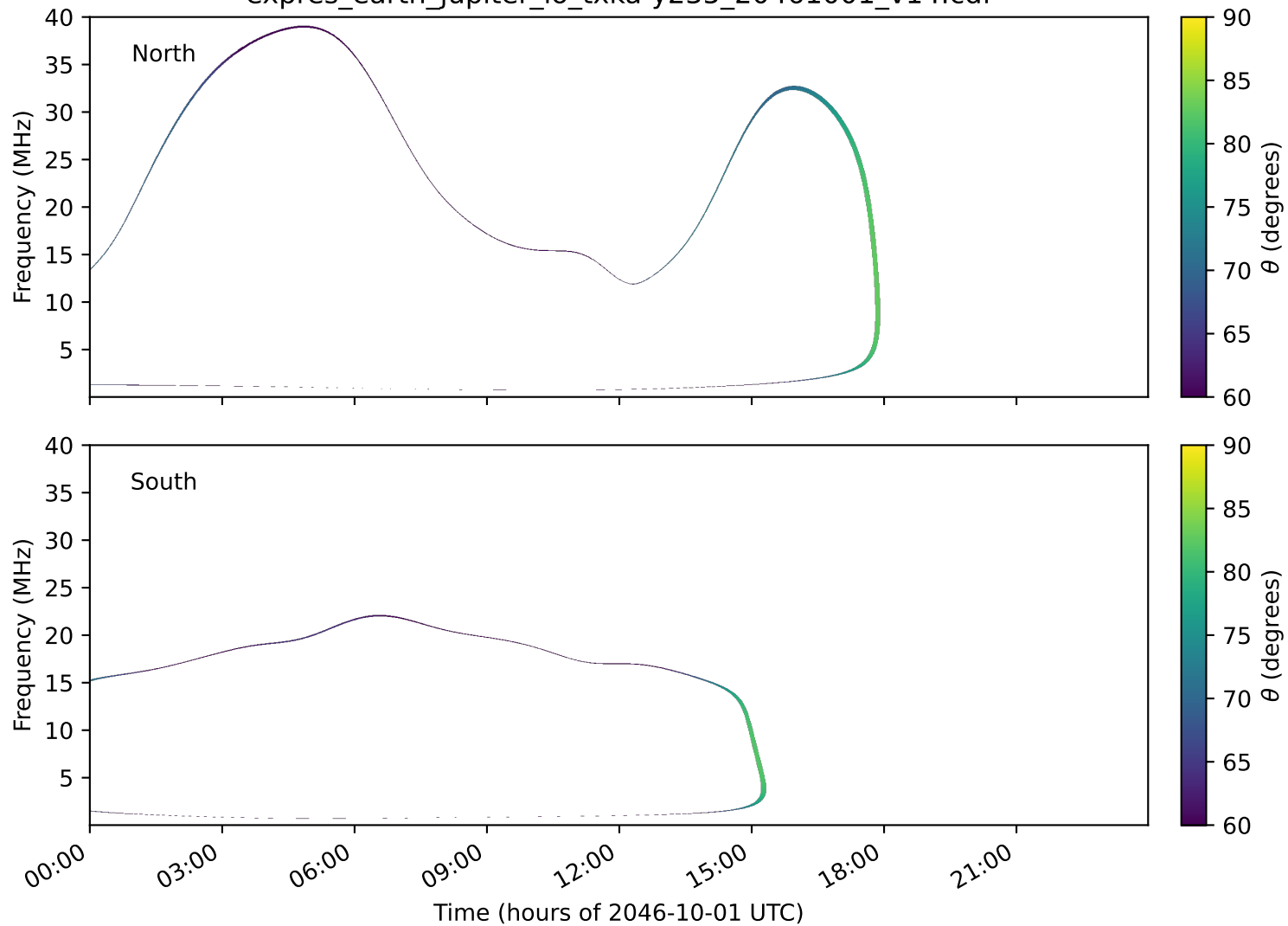
expres_earth_jupiter_io_txka-y235_20461001_v14.cdf
