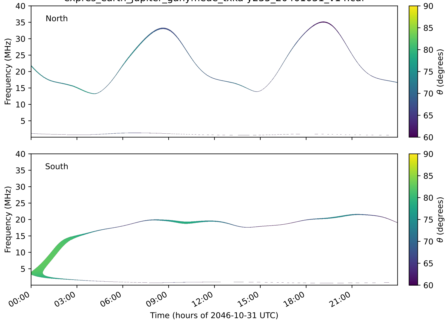
expres_earth_jupiter_ganymede_txka-y235_20461031_v14.cdf
