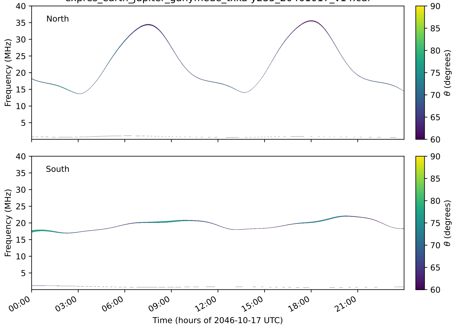
expres_earth_jupiter_ganymede_txka-y235_20461017_v14.cdf
