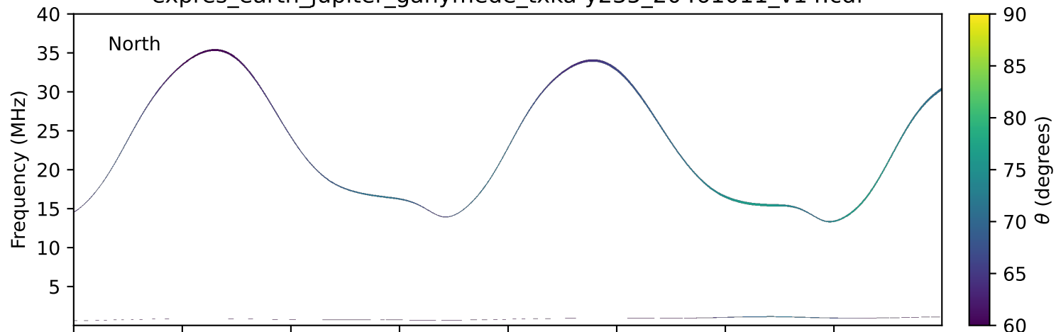
expres_earth_jupiter_ganymede_txka-y235_20461011_v14.cdf
