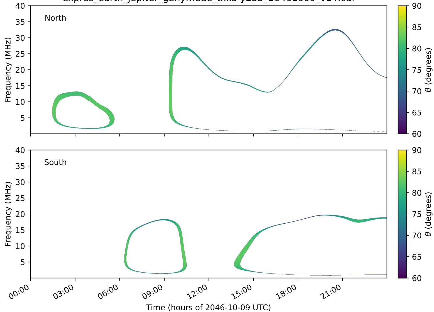
expres_earth_jupiter_ganymede_txka-y235_20461009_v14.cdf
