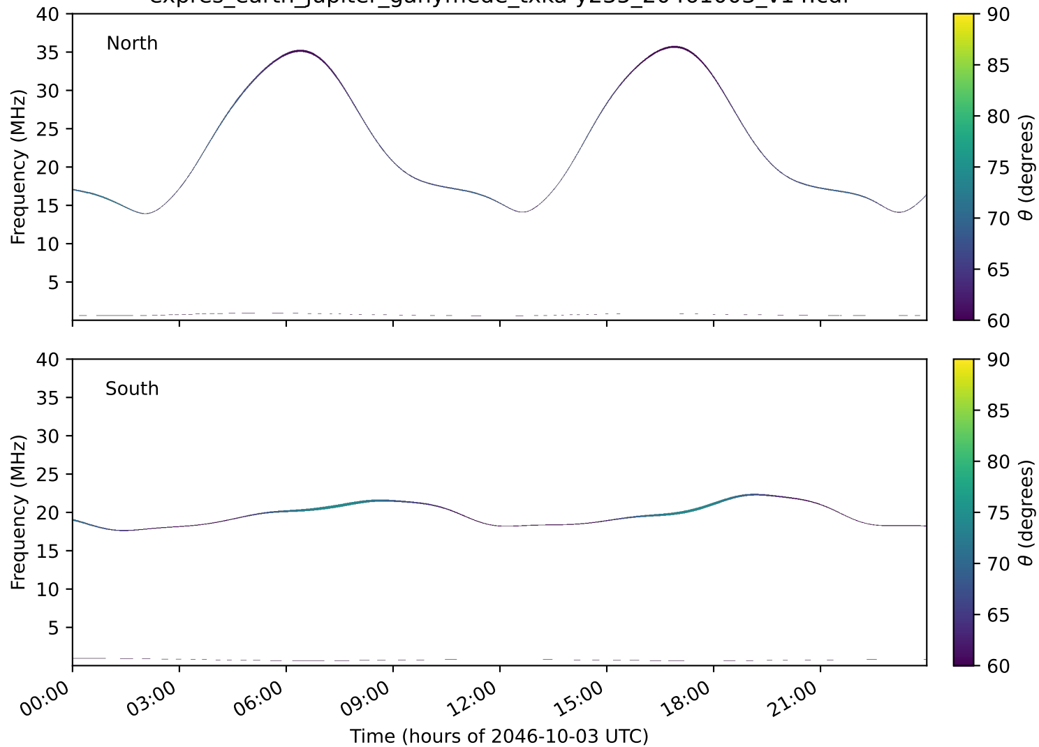
expres_earth_jupiter_ganymede_txka-y235_20461003_v14.cdf
