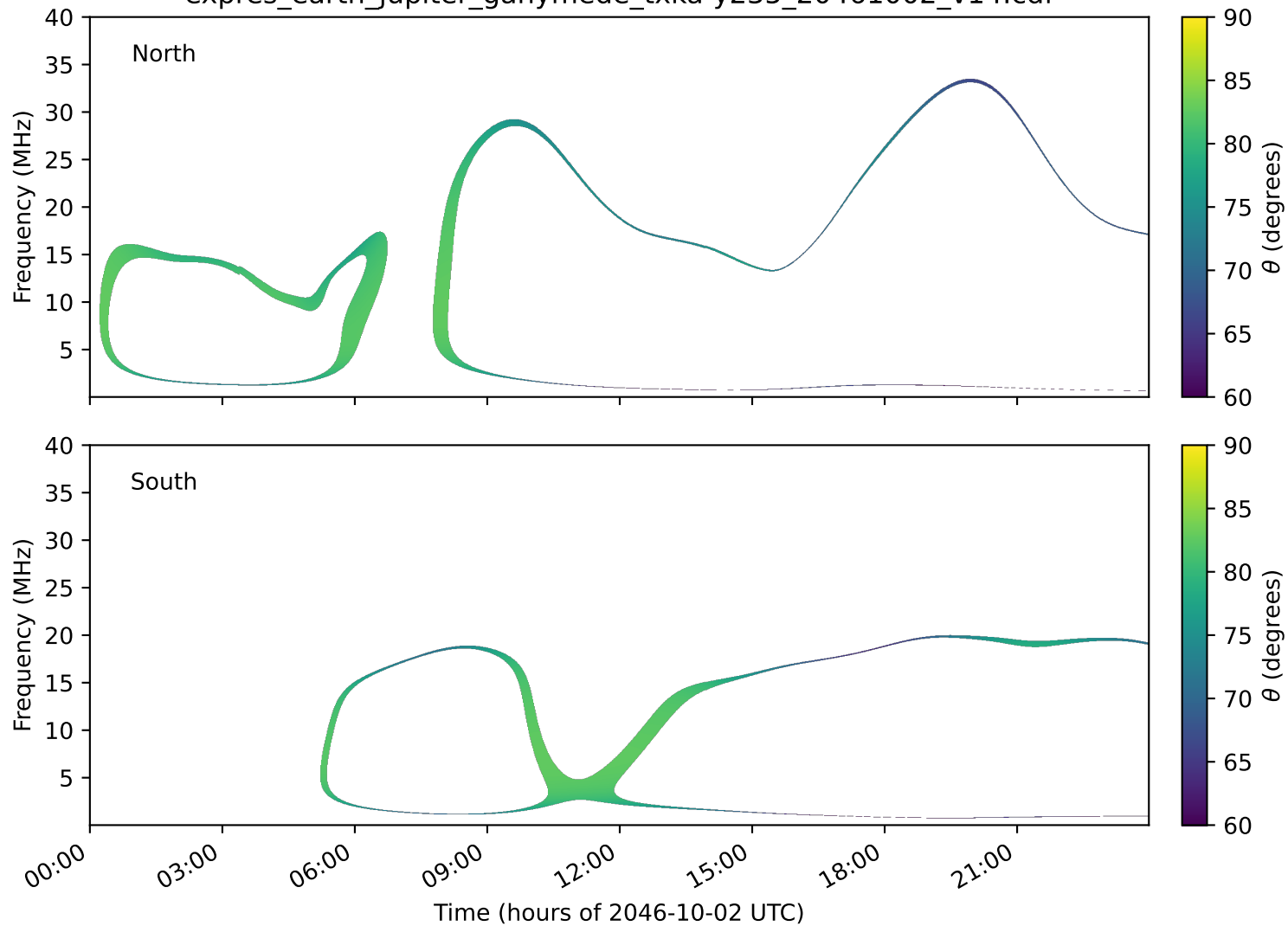
expres_earth_jupiter_ganymede_txka-y235_20461002_v14.cdf
