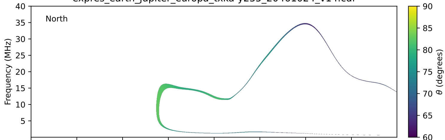
expres_earth_jupiter_europa_txka-y235_20461024_v14.cdf
