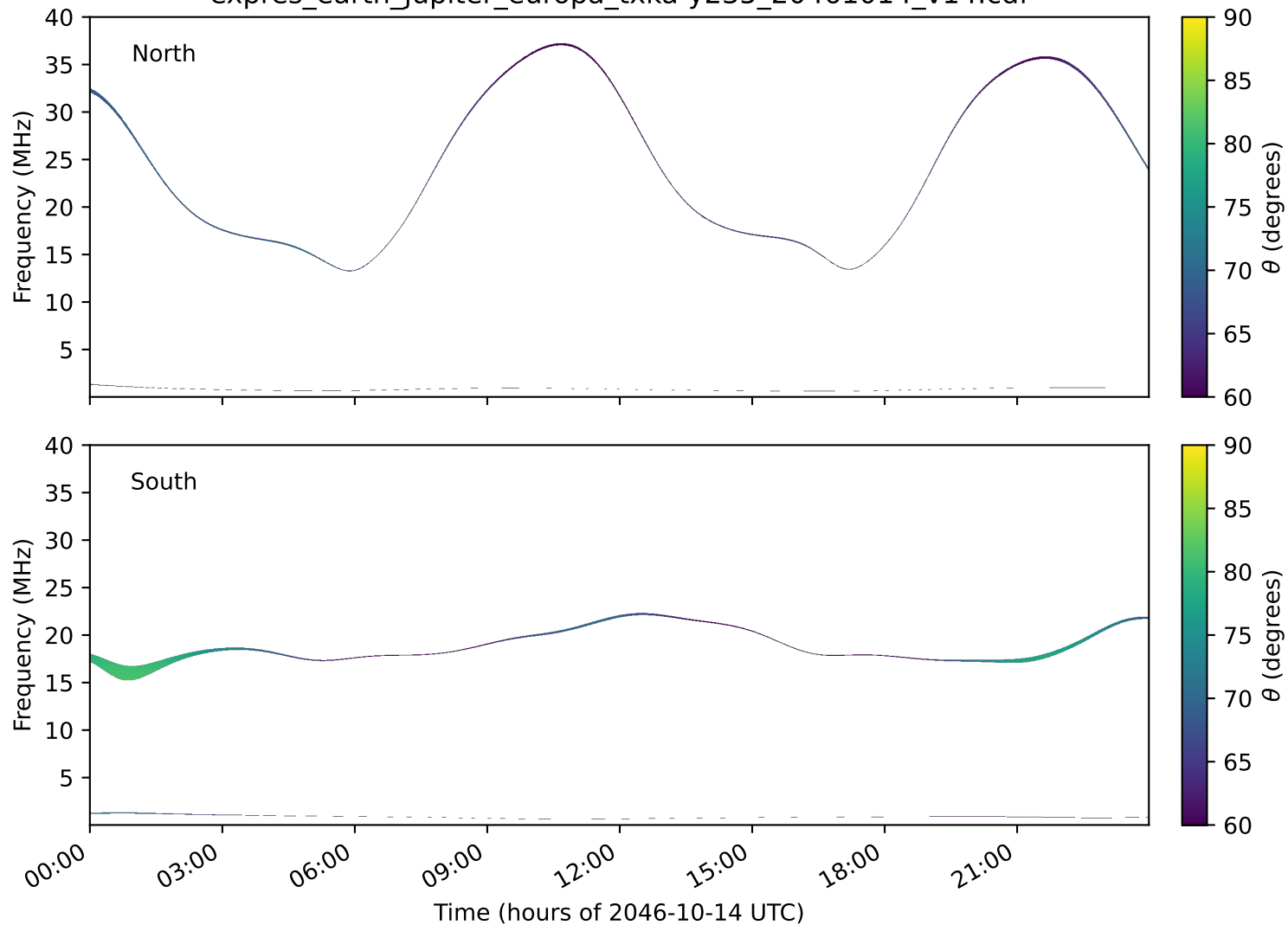
expres_earth_jupiter_europa_txka-y235_20461014_v14.cdf
