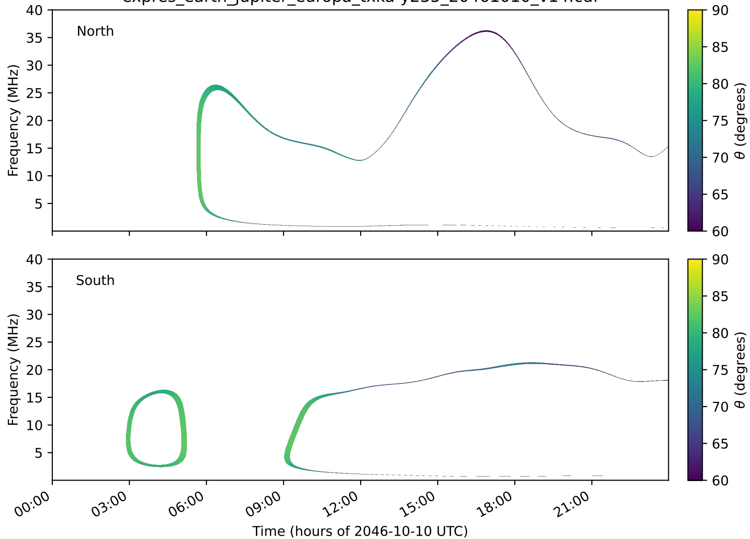
expres_earth_jupiter_europa_txka-y235_20461010_v14.cdf
