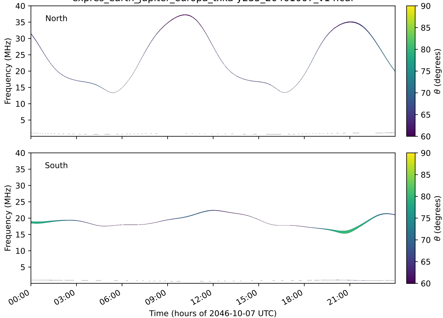
expres_earth_jupiter_europa_txka-y235_20461007_v14.cdf
