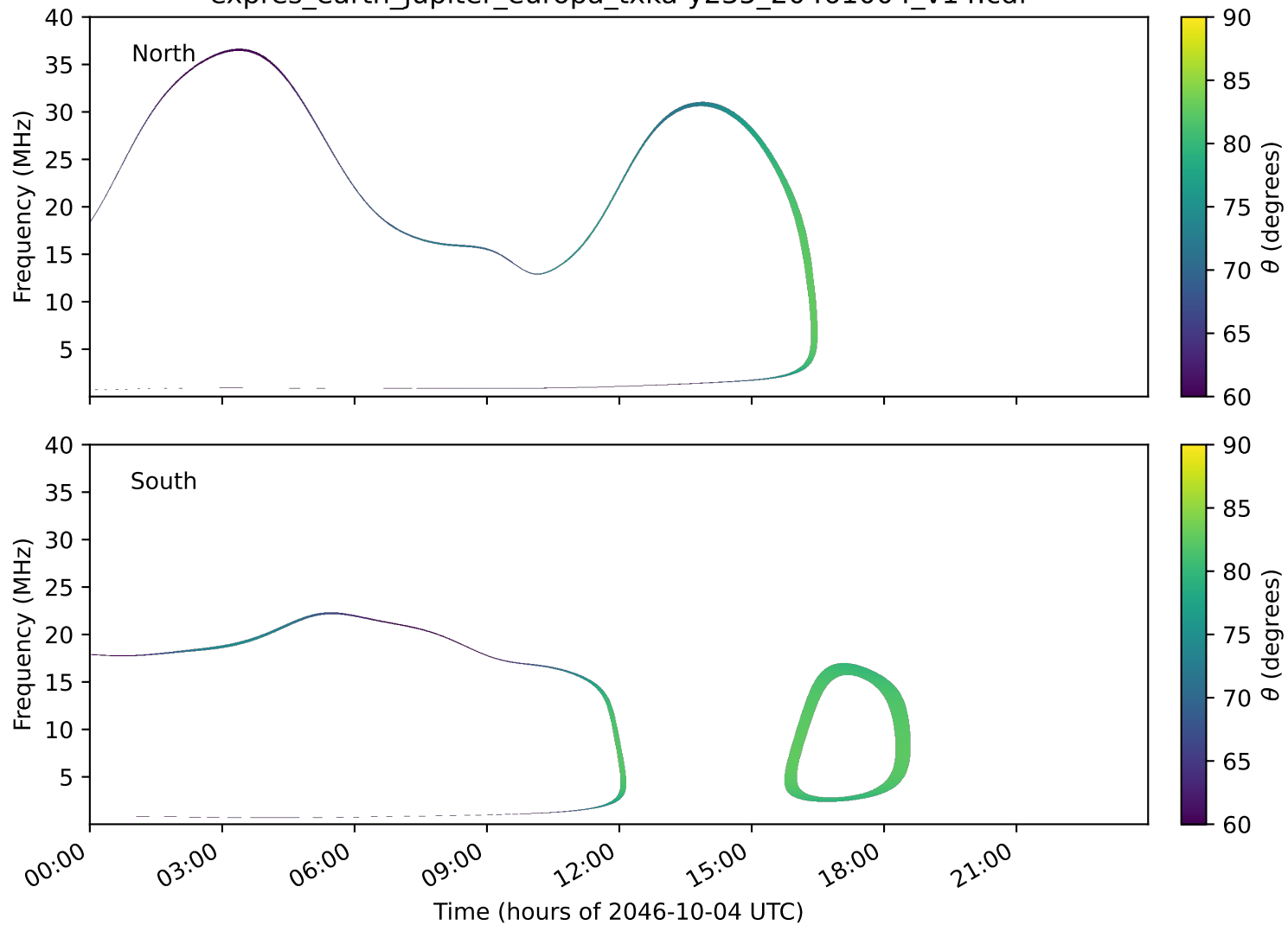
expres_earth_jupiter_europa_txka-y235_20461004_v14.cdf
