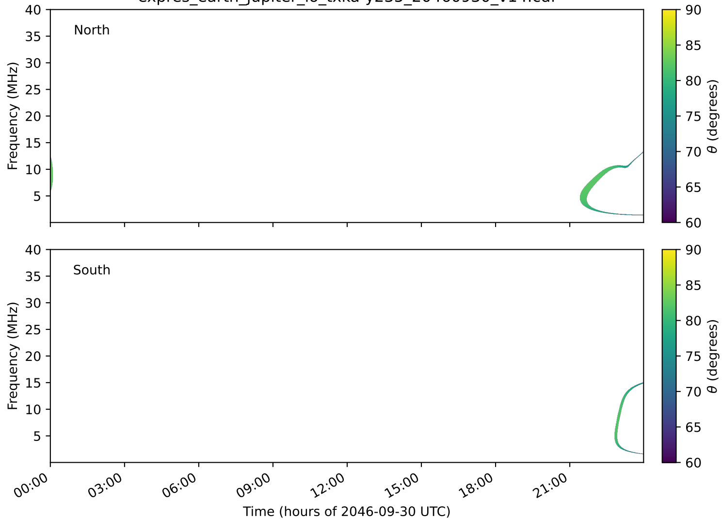
expres_earth_jupiter_io_txka-y235_20460930_v14.cdf
