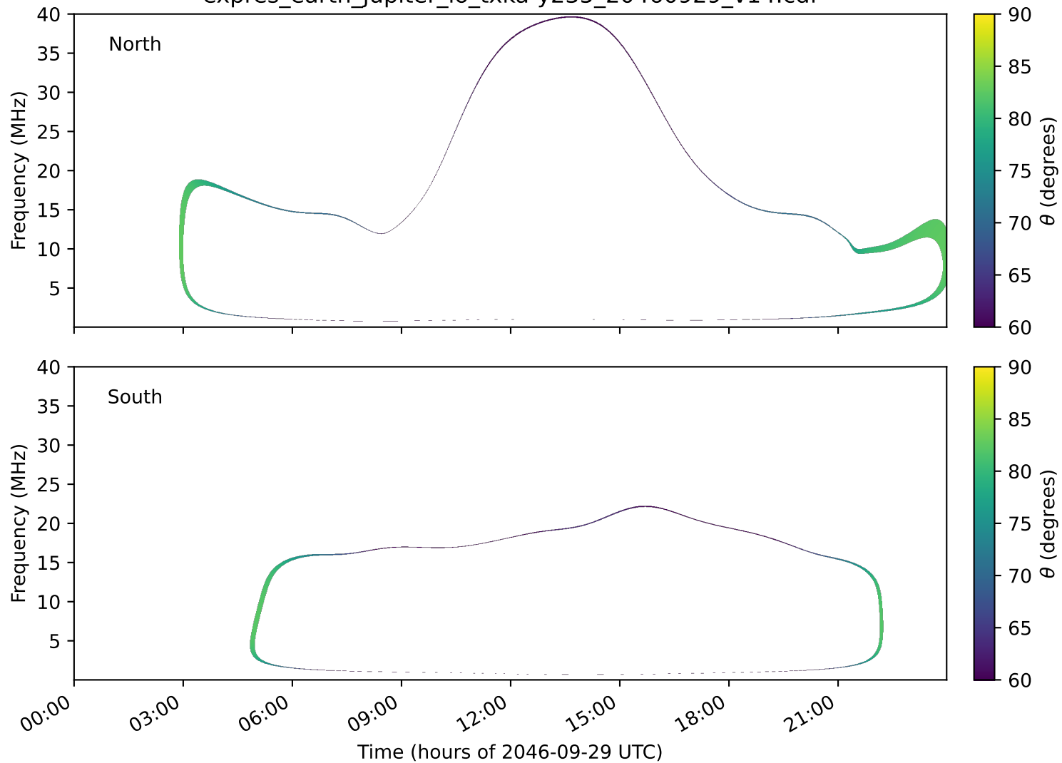
expres_earth_jupiter_io_txka-y235_20460929_v14.cdf
