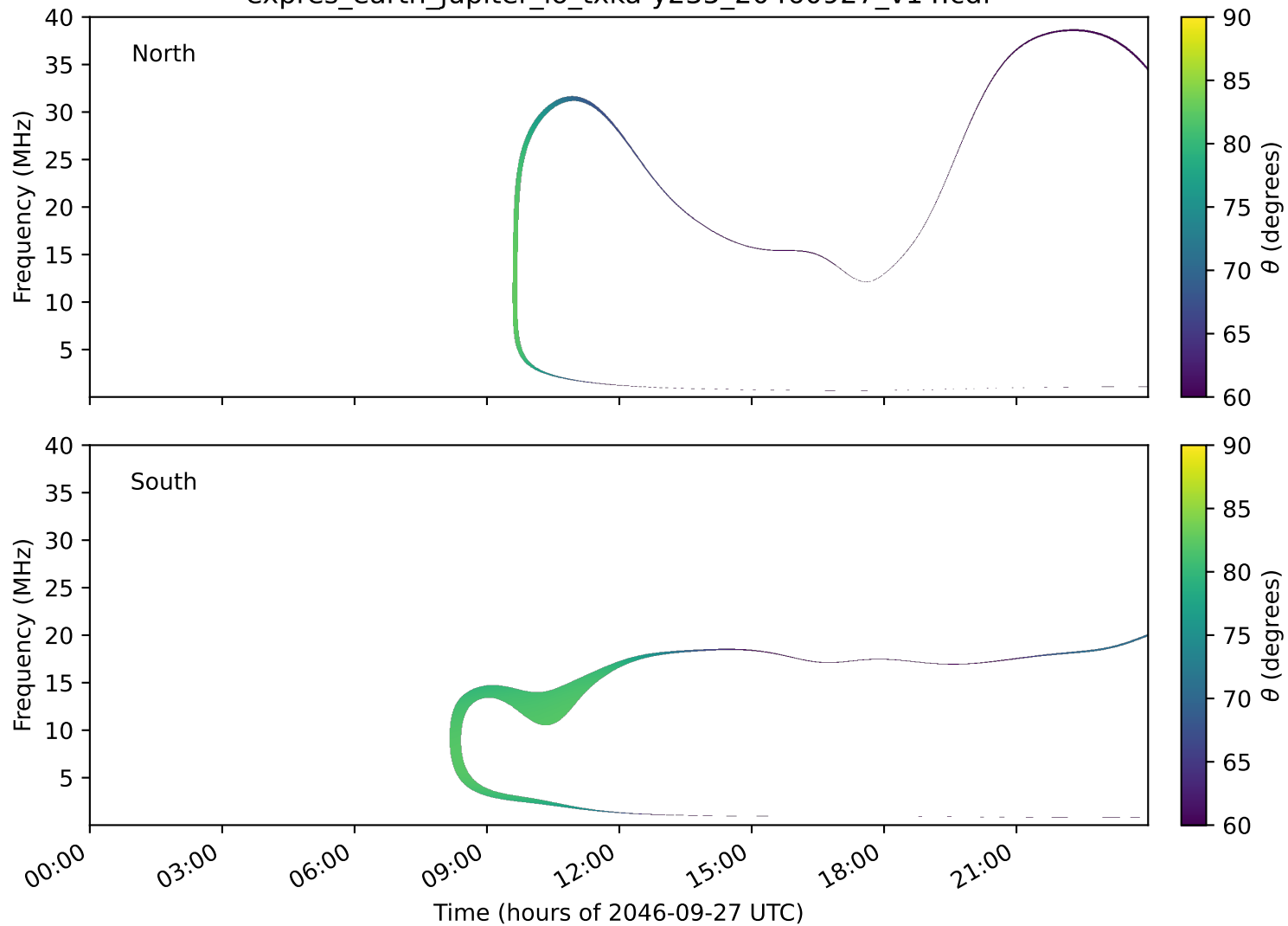
expres_earth_jupiter_io_txka-y235_20460927_v14.cdf
