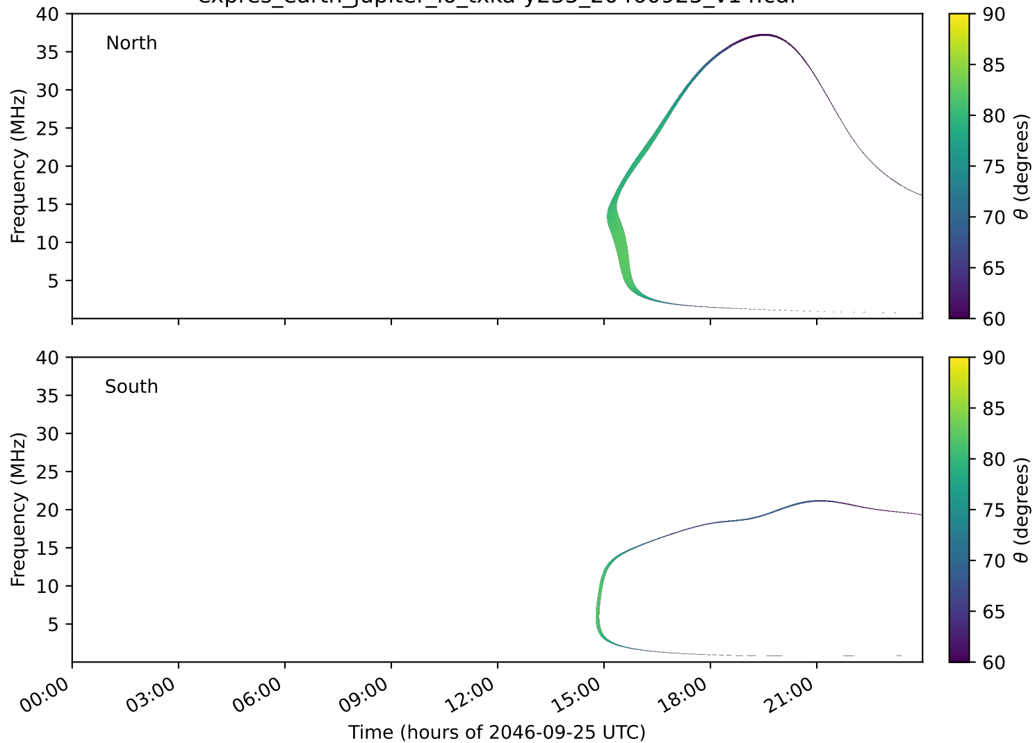
expres_earth_jupiter_io_txka-y235_20460925_v14.cdf
