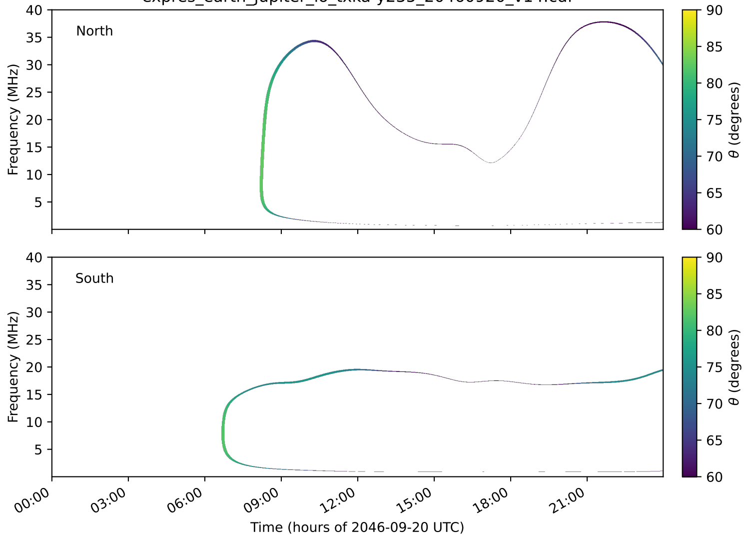
expres_earth_jupiter_io_txka-y235_20460920_v14.cdf
