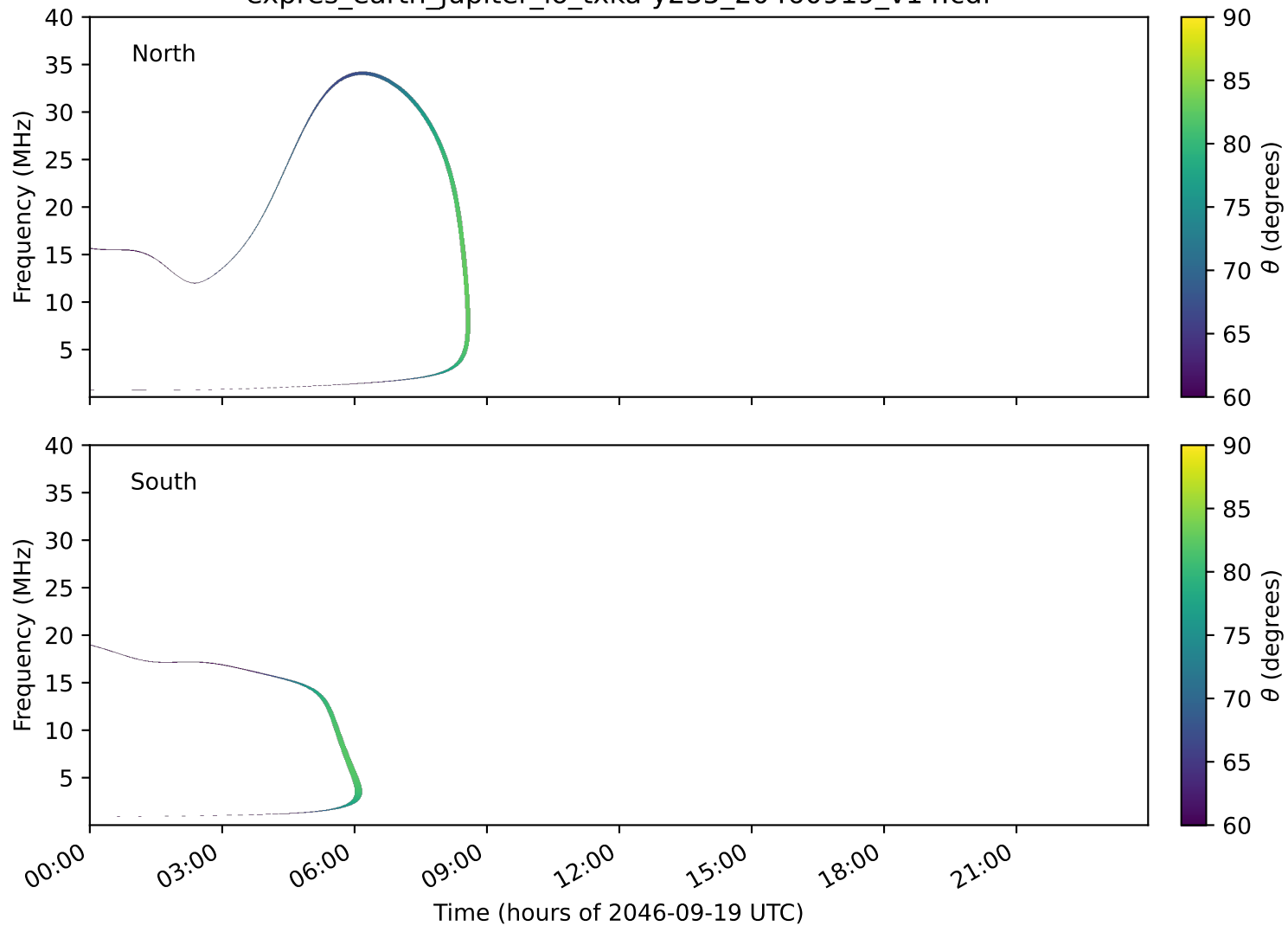
expres_earth_jupiter_io_txka-y235_20460919_v14.cdf
