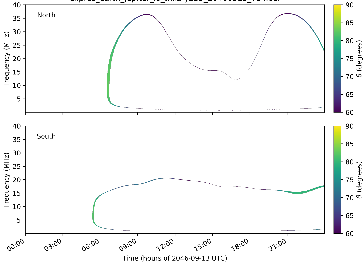
expres_earth_jupiter_io_txka-y235_20460913_v14.cdf
